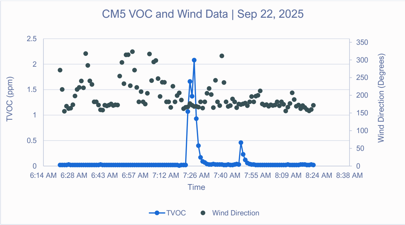
Figure 2 CM5 – Central Elementary School tVOC and Wind Direction September 22, 2025, 6:22 AM to 8:21 AM
