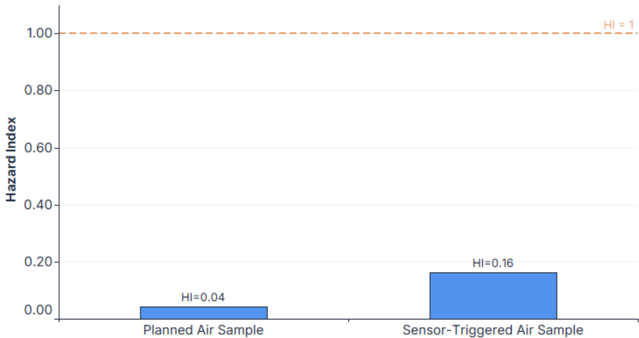
Figure 5 Hazard Indices at the CCND CM5 – Central Elementary School for Planned (August 27, 2025) and Sensor-Triggered (September 22, 2025) Air Samples
