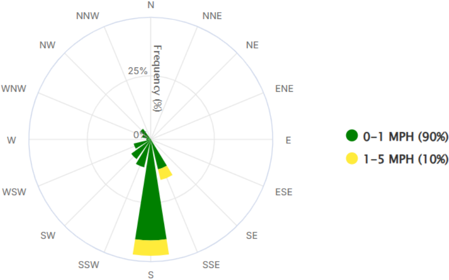
Figure 3 CM5 – Central Elementary School Wind Rose September 22, 2025, 6:22 AM to 8:21 AM
